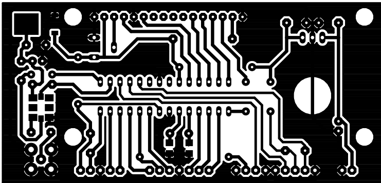
Digital Board (98x47mm, 1:1 A4 paper mirrored for Press and Peel)
