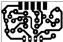
Serial Board (27x18mm, 1:1 A4 paper mirrored for Press and Peel)
