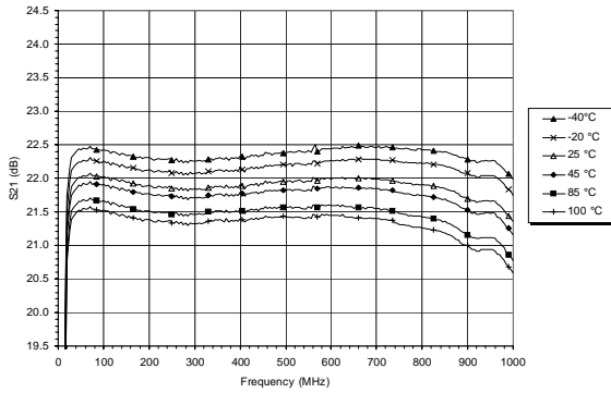
Figure 5: Gain / S21
