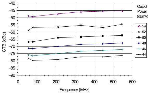
Figure 24: CTB (77 Channel Loading, Flat)
