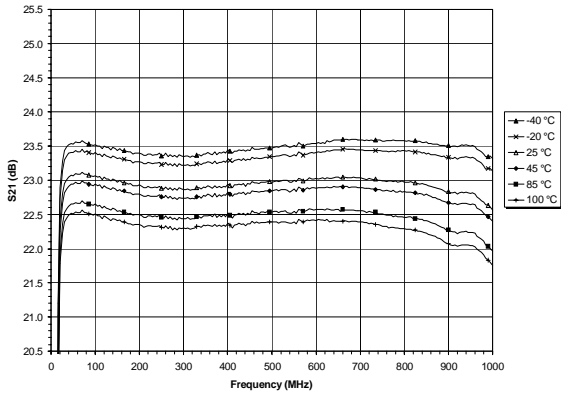
Figure 19: GAIN / S21
