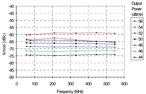
Figure 35: XMOD (77 Channel Loading, 8 dB Tilt)
