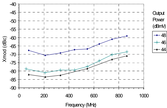
Figure 32: XMOD (128 Channel Loading, Flat)
