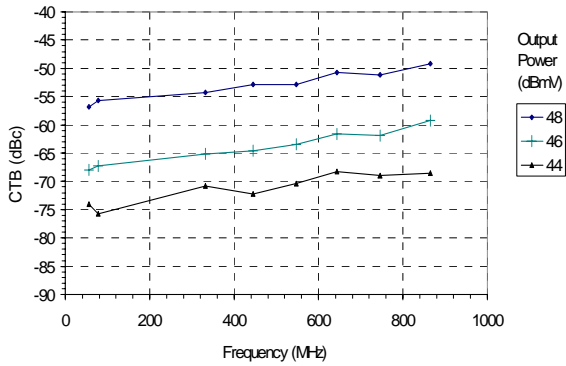
Figure 30: CTB (128 Channel Loading, Flat)
