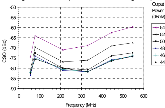
Figure 25: CSO (77 Channel Loading, Flat)
