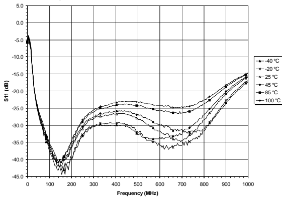
Figure 20: Input Return Loss / S11
