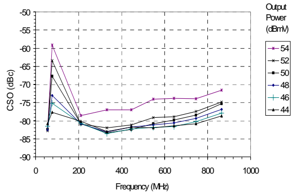
Figure 40: CSO (128 Channel Loading, 12 dB Tilt)
