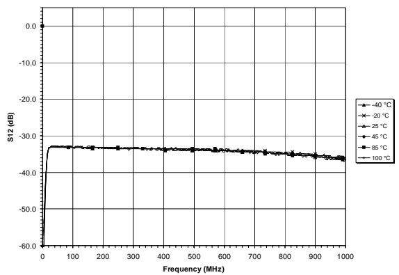
Figure 22: Reverse Isolation / S12
