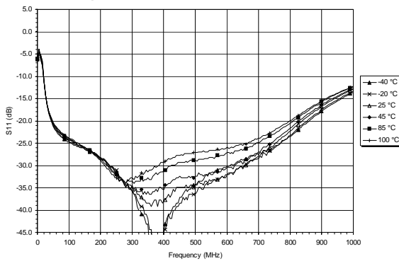
Figure 6: Input Return Loss / S11
