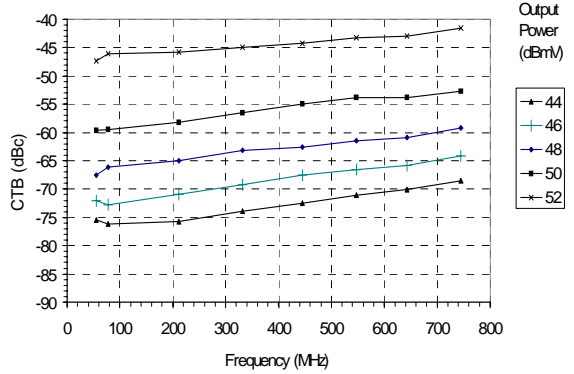
Figure 27: CTB (110 Channel Loading, Flat)
