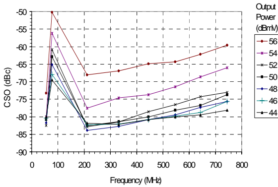
Figure 37: CSO (110 Channel Loading, 10 dB Tilt)
