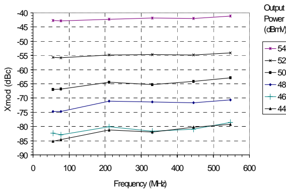
Figure 26: XMOD (77 Channel Loading, Flat)
