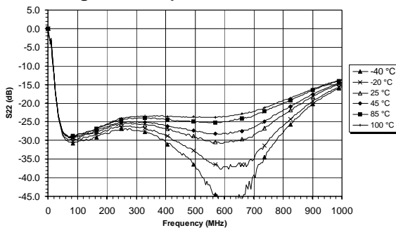
Figure 7: Output Return Loss / S22
