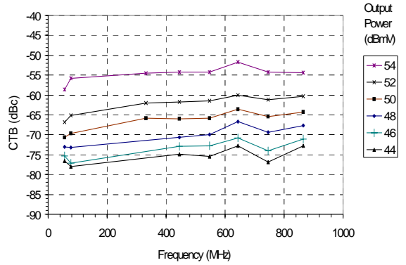
Figure 39: CTB (128 Channel Loading, 12 dB Tilt)
