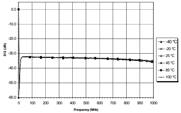
Figure 8: Reverse Isolation / S12
