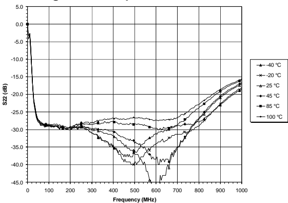
Figure 21: Output Return Loss / S22
