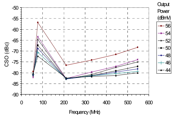
Figure 34: CSO (77 Channel Loading, 8 dB Tilt)
