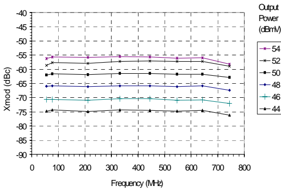
Figure 38: XMOD (110 Channel Loading, 10 dB Tilt)
