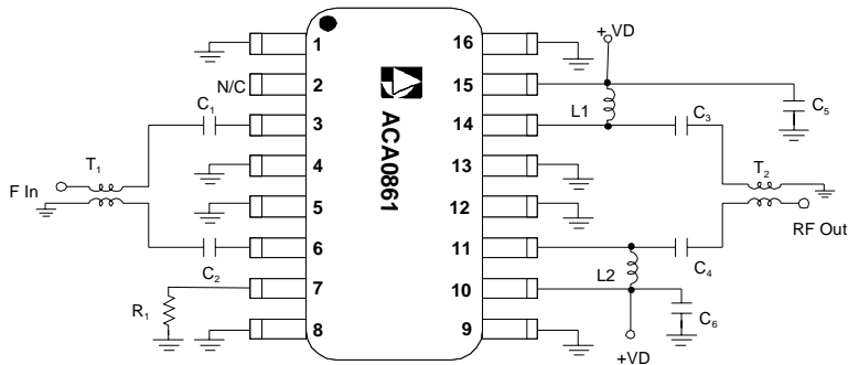
Figure 3: Test Circuit
