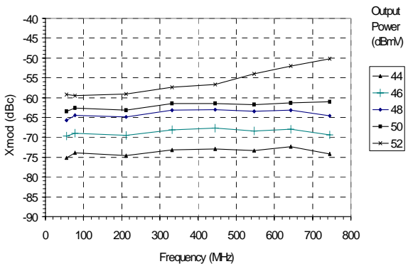
Figure 29: XMOD (110 Channel Loading, Flat)
