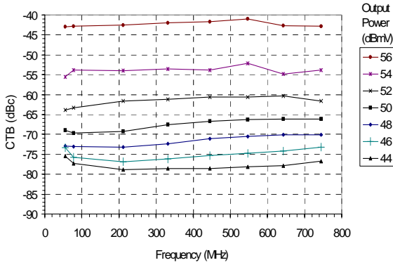
Figure 36: CTB (110 Channel Loading, 10 dB Tilt)
