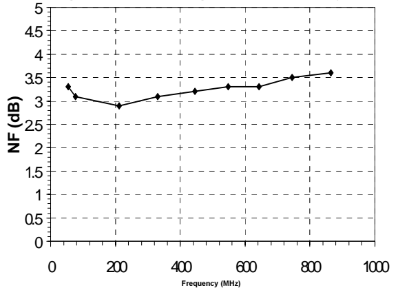
Figure 23: Noise Figure vs. Frequency
