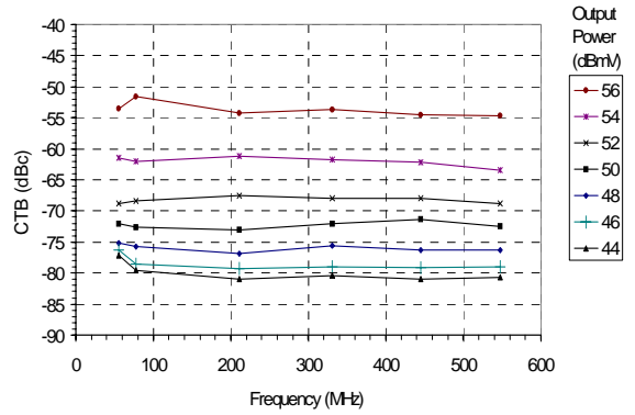
Figure 33: CTB (77 Channel Loading, 8 dB Tilt)
