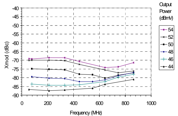
Figure 41: XMOD (128 Channel Loading, 12 dB Tilt)
