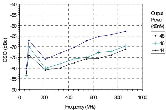
Figure 31: CSO (128 Channel Loading, Flat)
