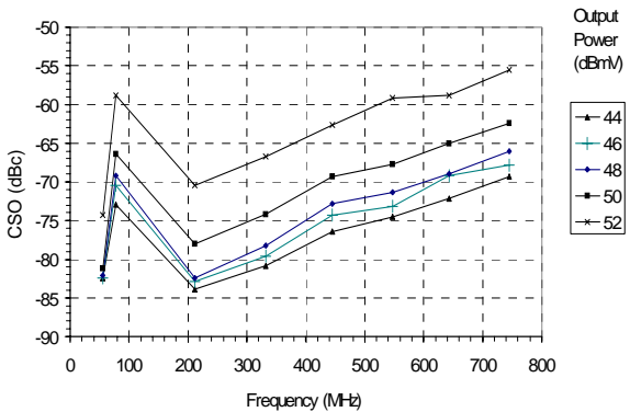
Figure 28: CSO (110 Channel Loading, Flat)
