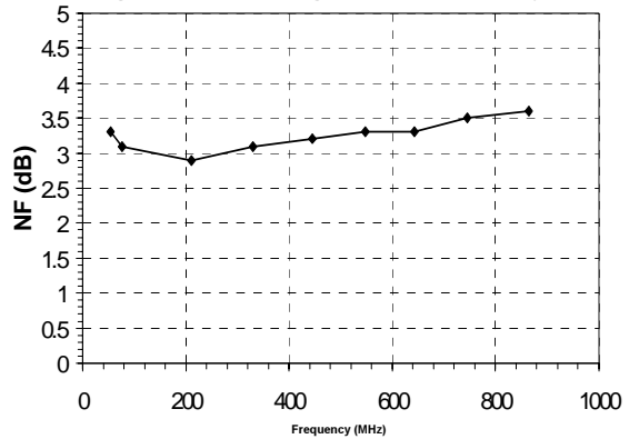
Figure 9: Noise Figure vs. Frequency
